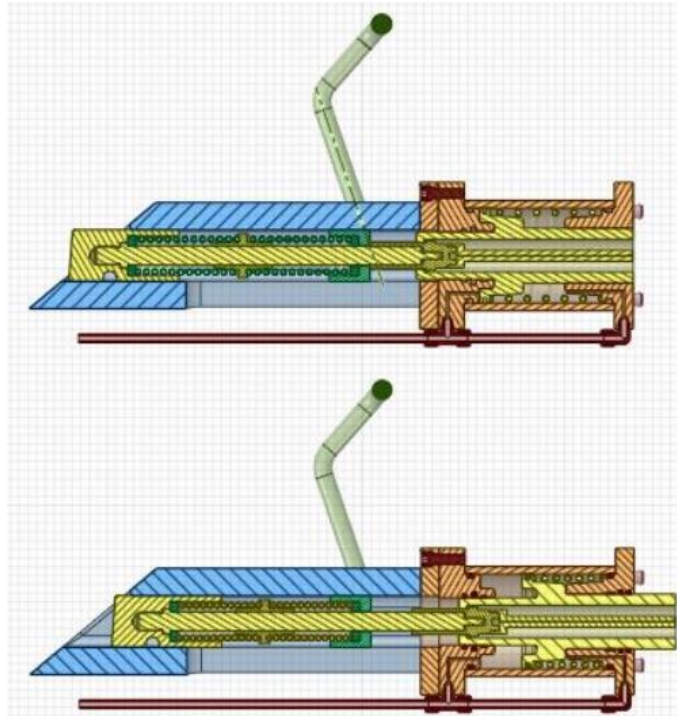
Figure 13: Hydraulic Actuation
