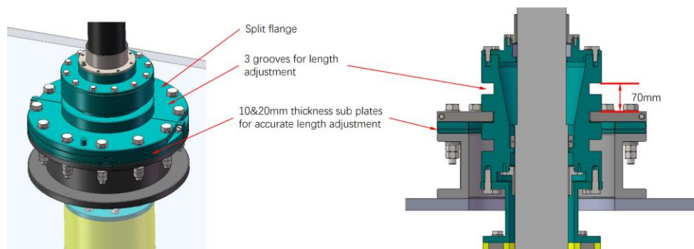
Figure 20: Hang off design with length adjustment
