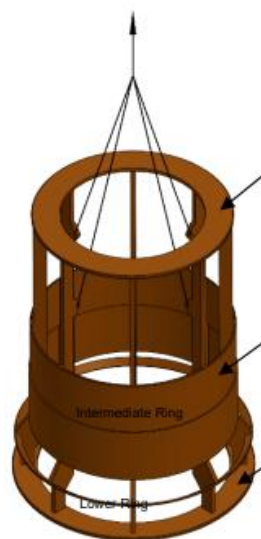
Figure 41: Dummy Cap - Template for the TSUDL Flexible Riser Pull-In Simulation Tests
