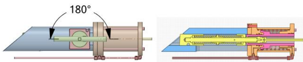
Figure 12: 180° rotation performed by lateral detachable handler
