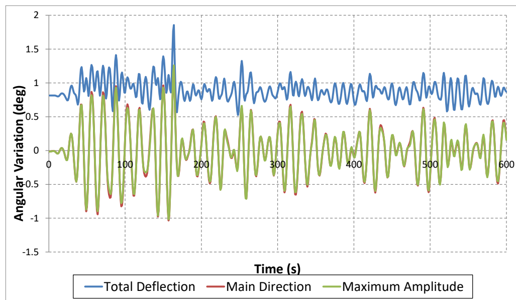
Figure 16 – Angular variation curves
