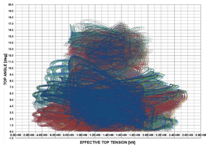
Figure 10 – Plot example of Tension x Top angle
