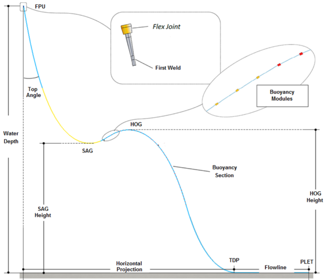
Figure 1 – SLWR Configuration
