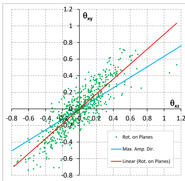
Figure 15 – Directions for angular variation calculation.
