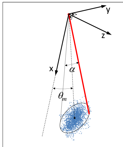
Figure 11 – Eccentric angular variation
