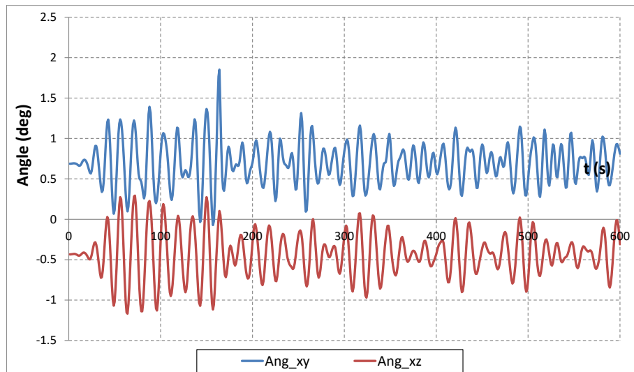
Figure 13 – Angular variation curves on X-Y and X-Z planes
