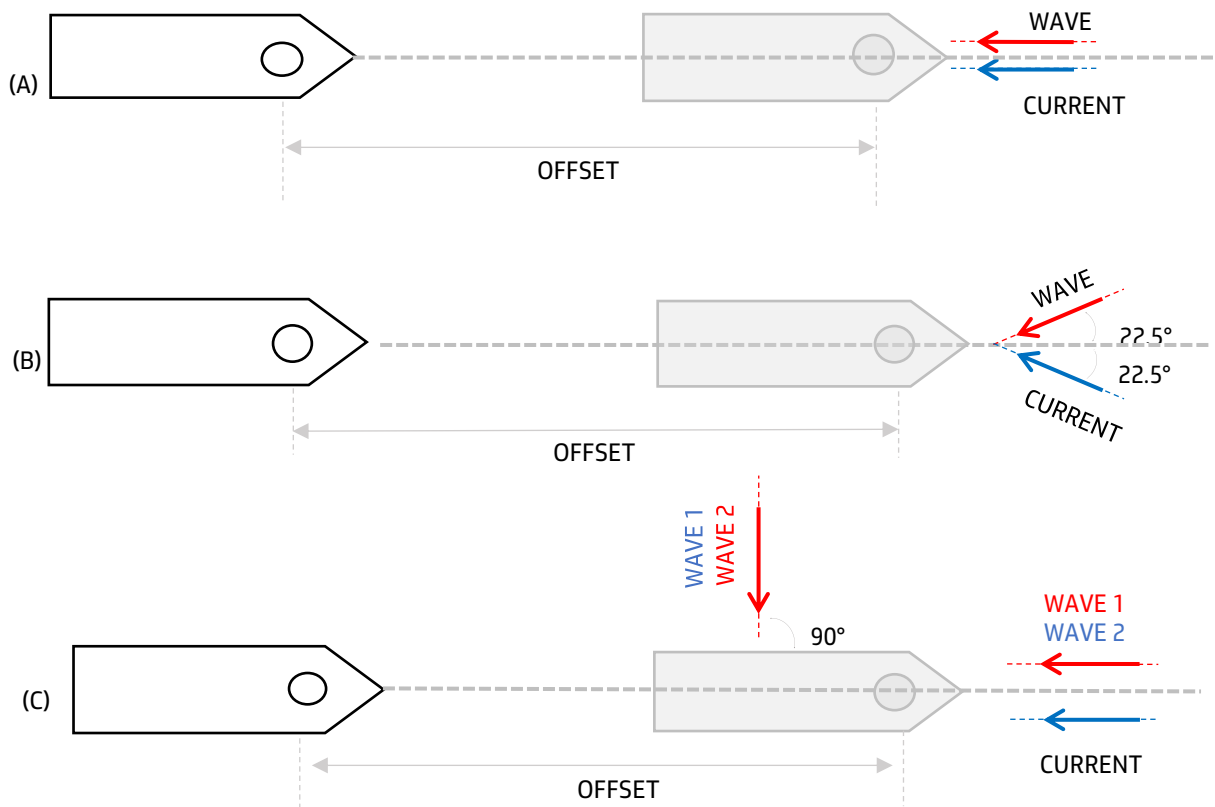
Figure 3 – Environmental conditions for SPM FPUs: (A) Head seas (b) Quartering seas (c) Beam seas
