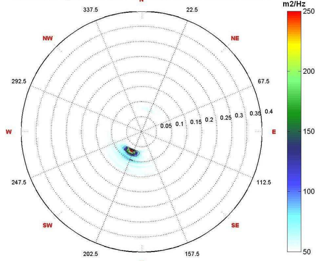
Figure 5.1.1 Typical single peak spectrum from SW-S quadrant wave storm
