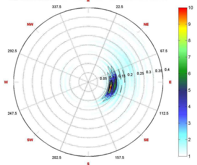
Figure 5.1.2 Typical single peak spectrum from E wave conditions
