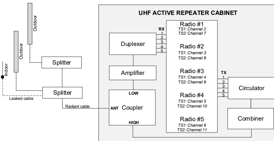
Figure 2: typical UHF active repeater system
