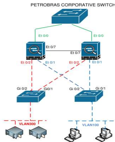
Figure 15: typical topology for 3 rd parties access
