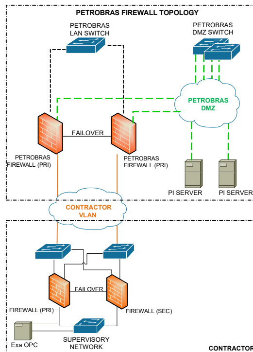
Figure 6: PETROBRAS PI interconnections to CONTRACTOR
