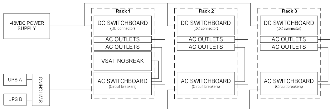
Figure 10: schematic power arrangement for PETROBRAS racks
