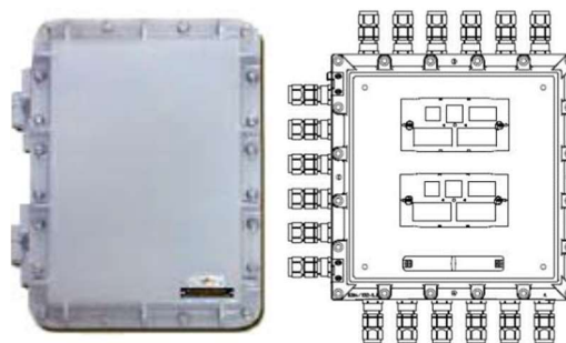
Figure 12: typical Ex-d Junction Box
