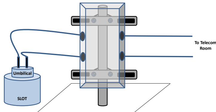
Figure 11: typical JB arrangement
