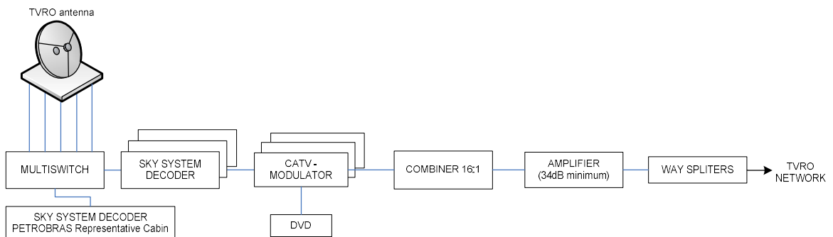
Figure 4: TVRO system general arrangement
