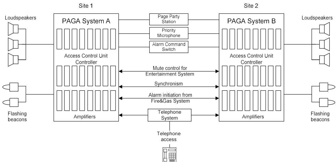
Figure 3: PAGA system general arrangement
