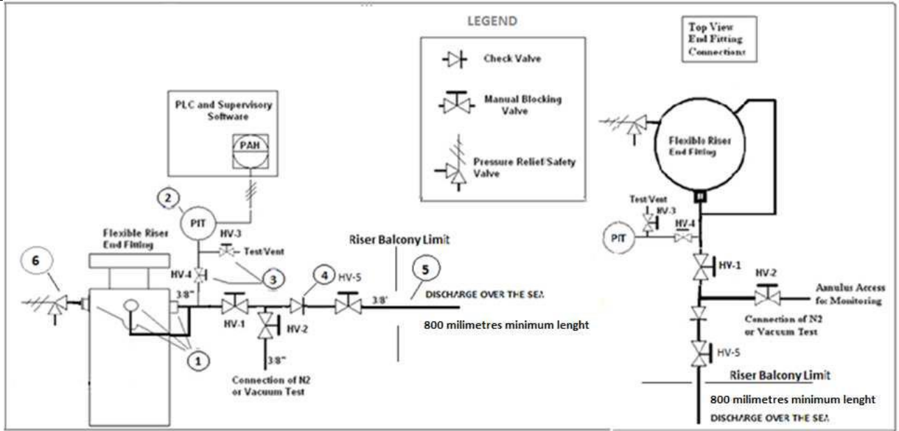
Figure 6.2 – Basic Diagram for the Local Continuous Vented Type
