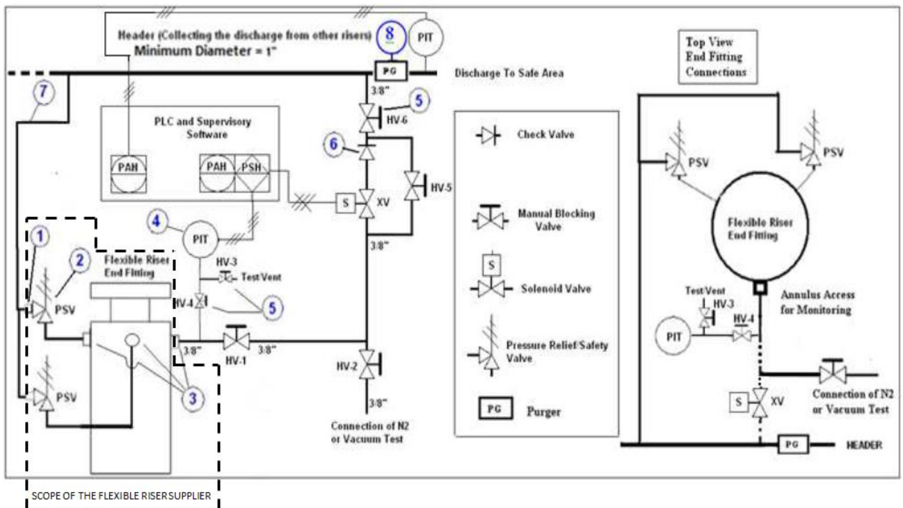
Figure 4.2 – Basic Diagram for the Automatic Type
