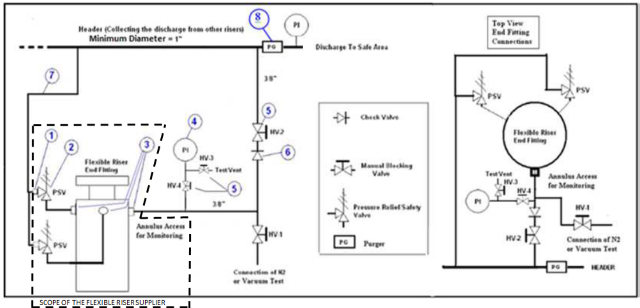
Figure 5.1 – Basic Diagram for the Manual Annulus Monitoring and Relief System
