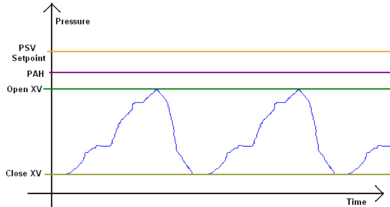
Figure 4.1 – Annulus Pressure behavior over time and set points
