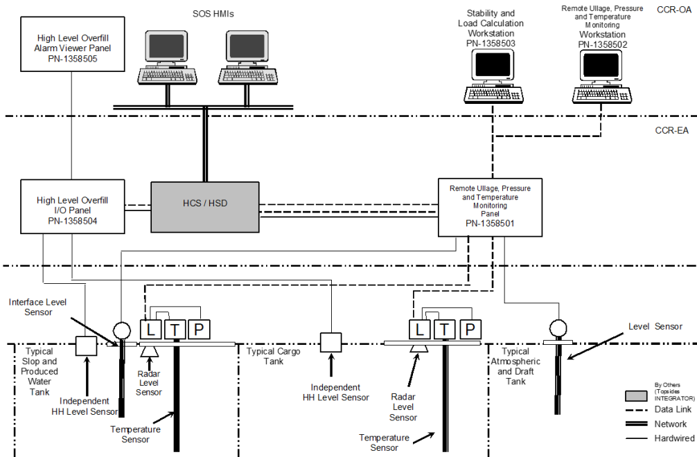
Figure 1 – HSTS Automation Architecture
