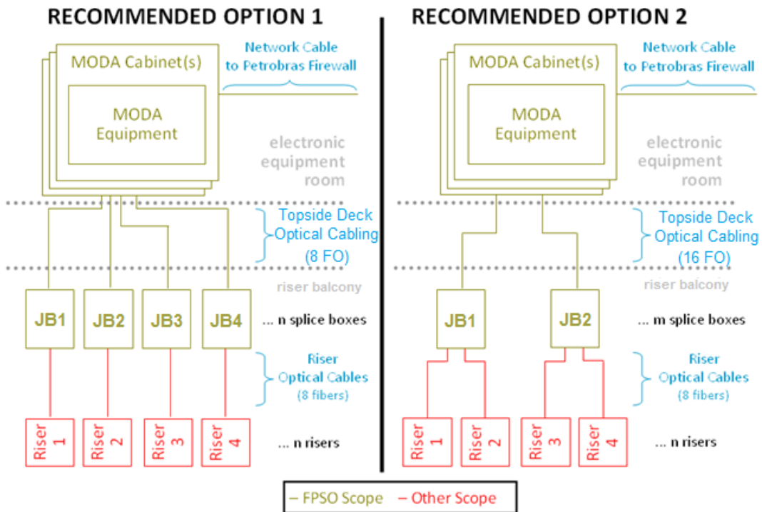
Figure 6 – MODA recommended layout options.
