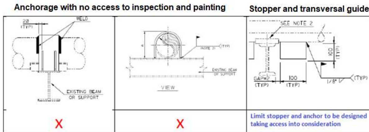
Figure 12 – Example of welded clamp that shall not be used (a) and (b). Example of appropriate limit stopper (c)
