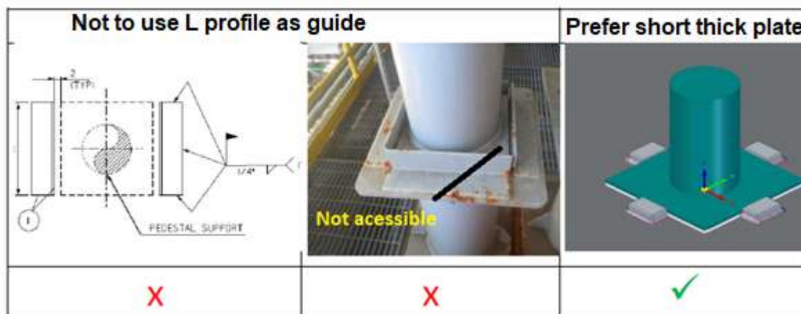
Figure 4 – Design of guide support that shall be avoided (a) and (b), and design that is preferrable (c)
