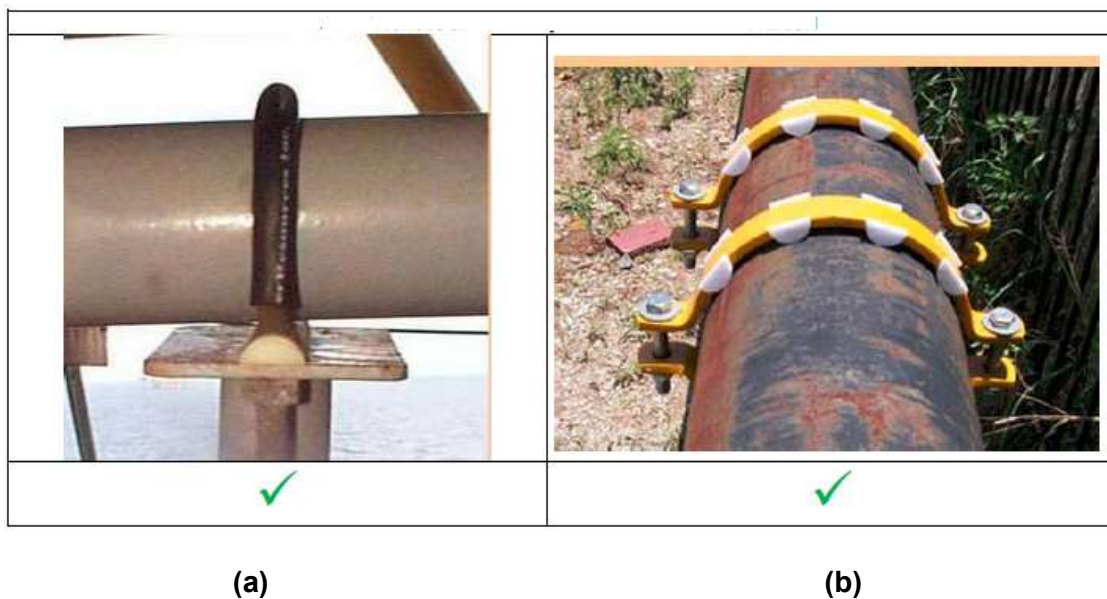
Figure 13 – Example of preferable types of contact between U-bolt and pipe (a) and clamps and pipe (b)
