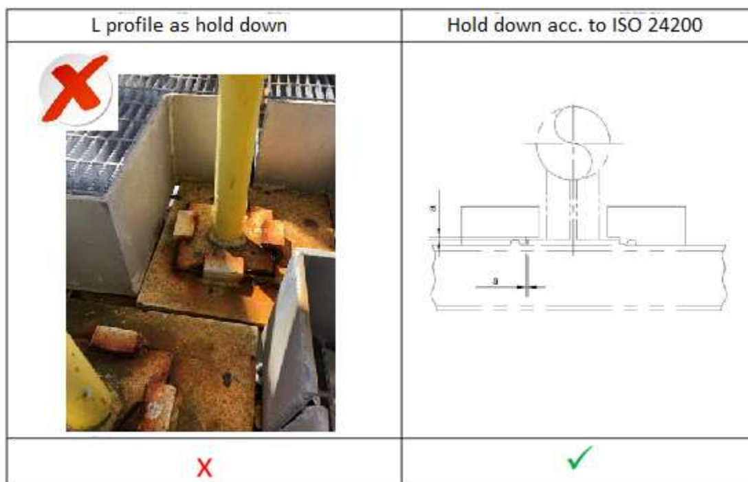
Figure 5 – Design of hold-down support that shall be avoided (a) and (b), and design that is preferrable (c)
