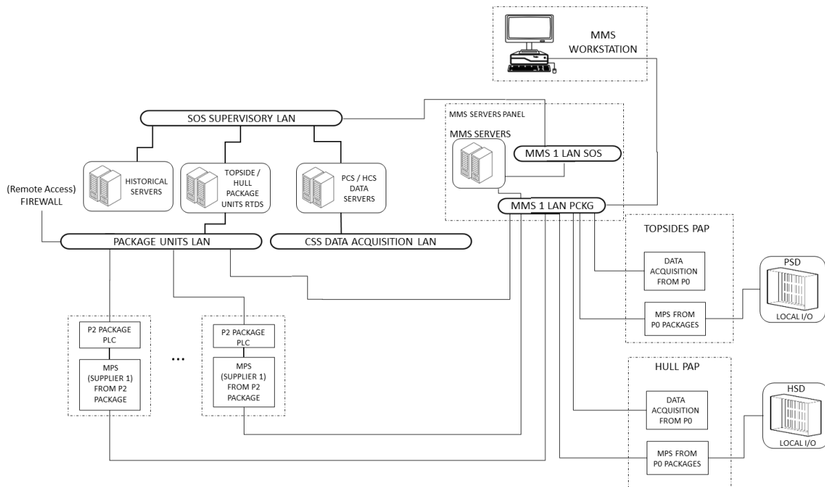
FIGURE 2 – MMS ARCHITECTURE
