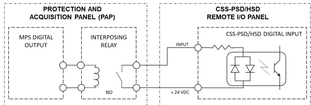
FIGURE 1 - INTERPOSING RELAY FOR SIGNALS FROM MPS TO CSS-PSD/HSD.
