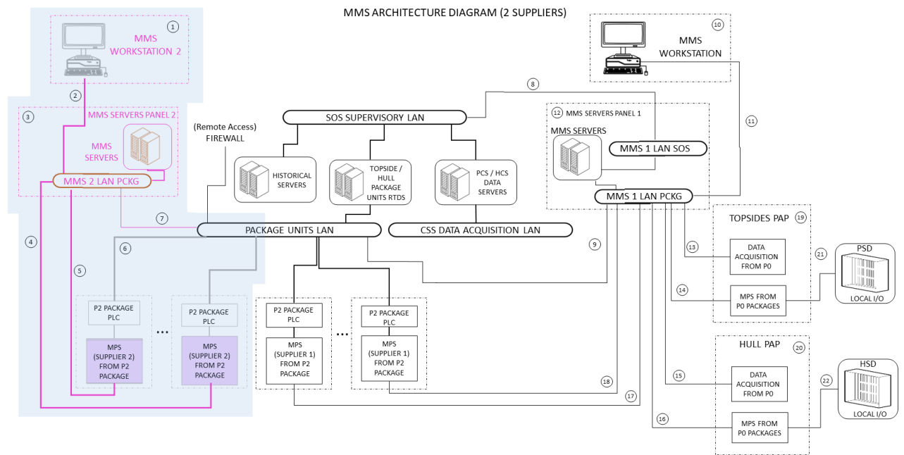
FIGURE 4 – OFFSHORE ACCESS TO MULTIPLE MMS SERVERS
