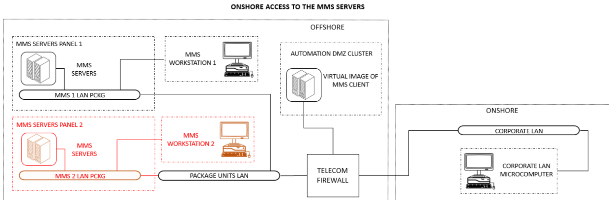
FIGURE 5 – ONSHORE ACCESS TO MULTIPLE MMS SERVERS
