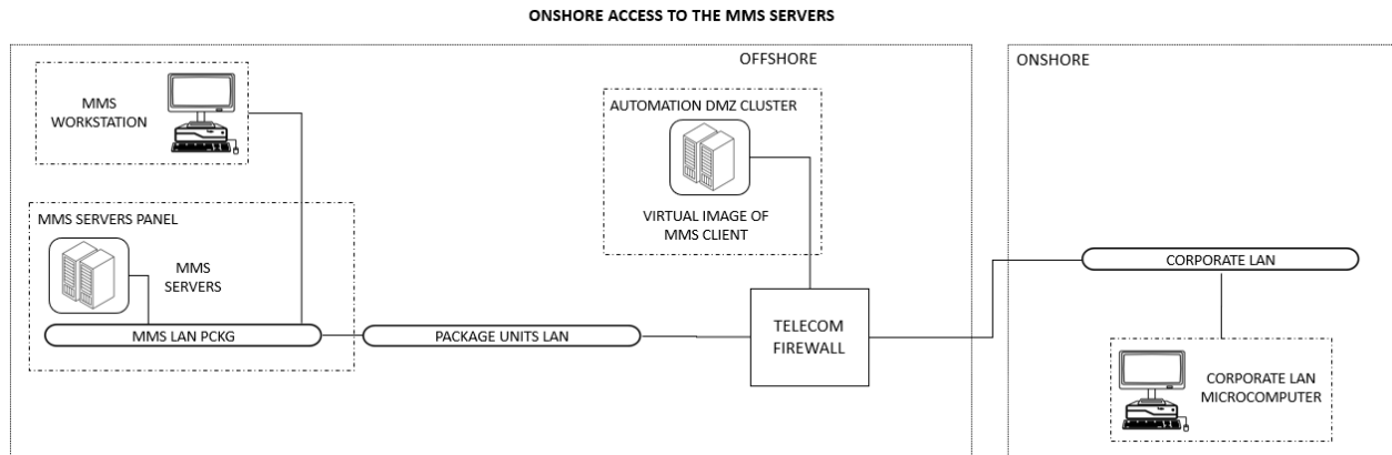
FIGURE 3 – ONSHORE ACCESS TO THE MMS SERVER
