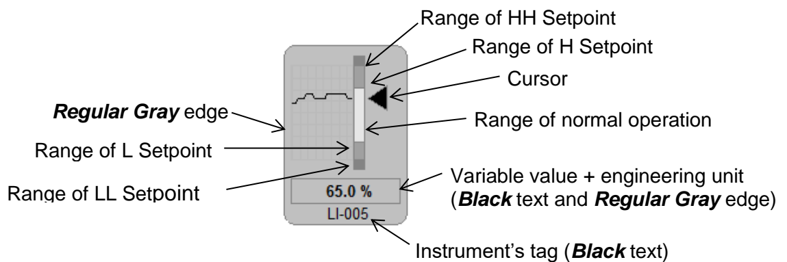
Figure 36 – General Transmitter.
