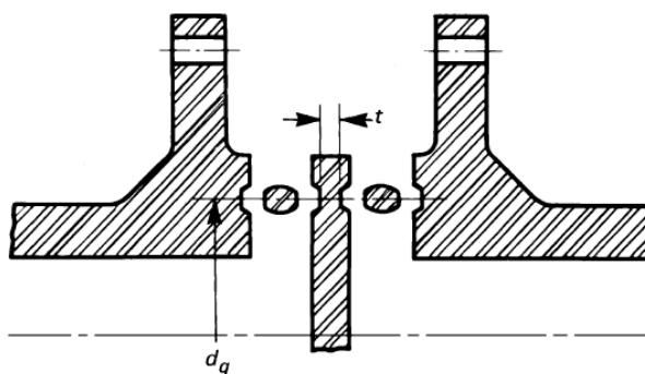
Figure L1 – Type of blank applied to API 6A flanges (REF.: ASME B31.3 para. 304.5.3).
