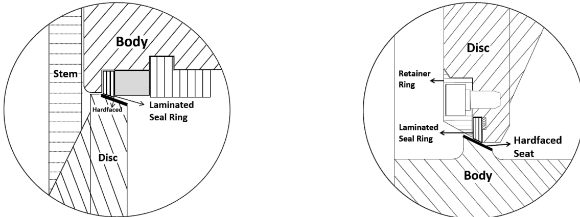
(a) Seal ring fixed to body & hard coating on disc
