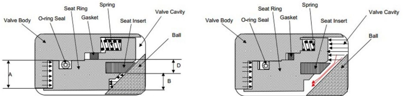
Figure A.4 – SPE/SR seat assembly mechanism (illustration on a soft ball valve)
