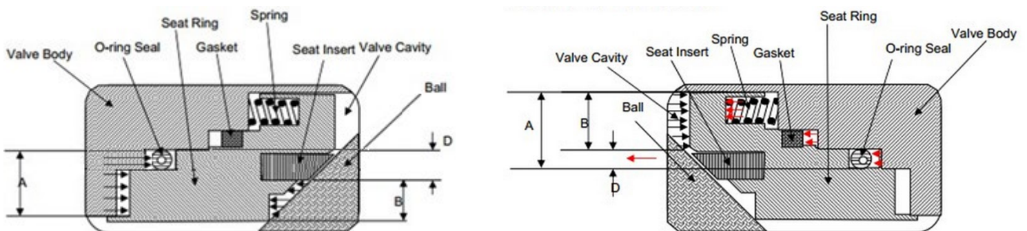
Figure A.5 – DPE seat assembly mechanism (illustration on a soft ball valve)
