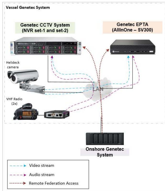
Figure-3 – ETEX recording system streams
