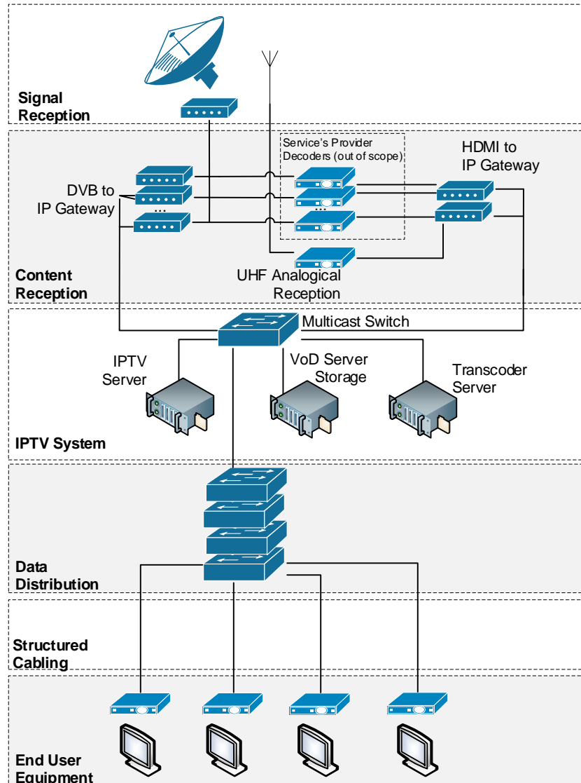
Figure 2: TVRO Architecture
